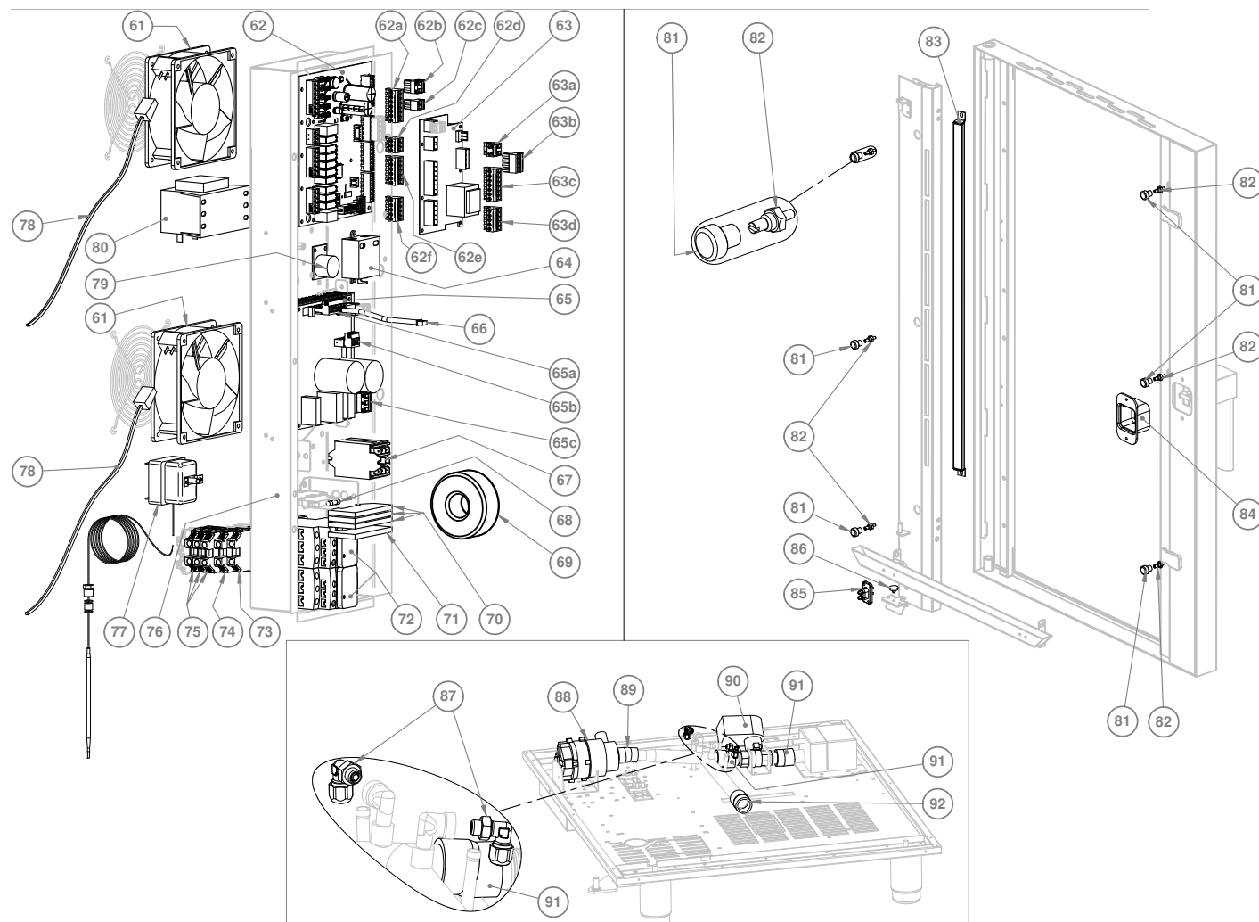
Exploded view 2/2
