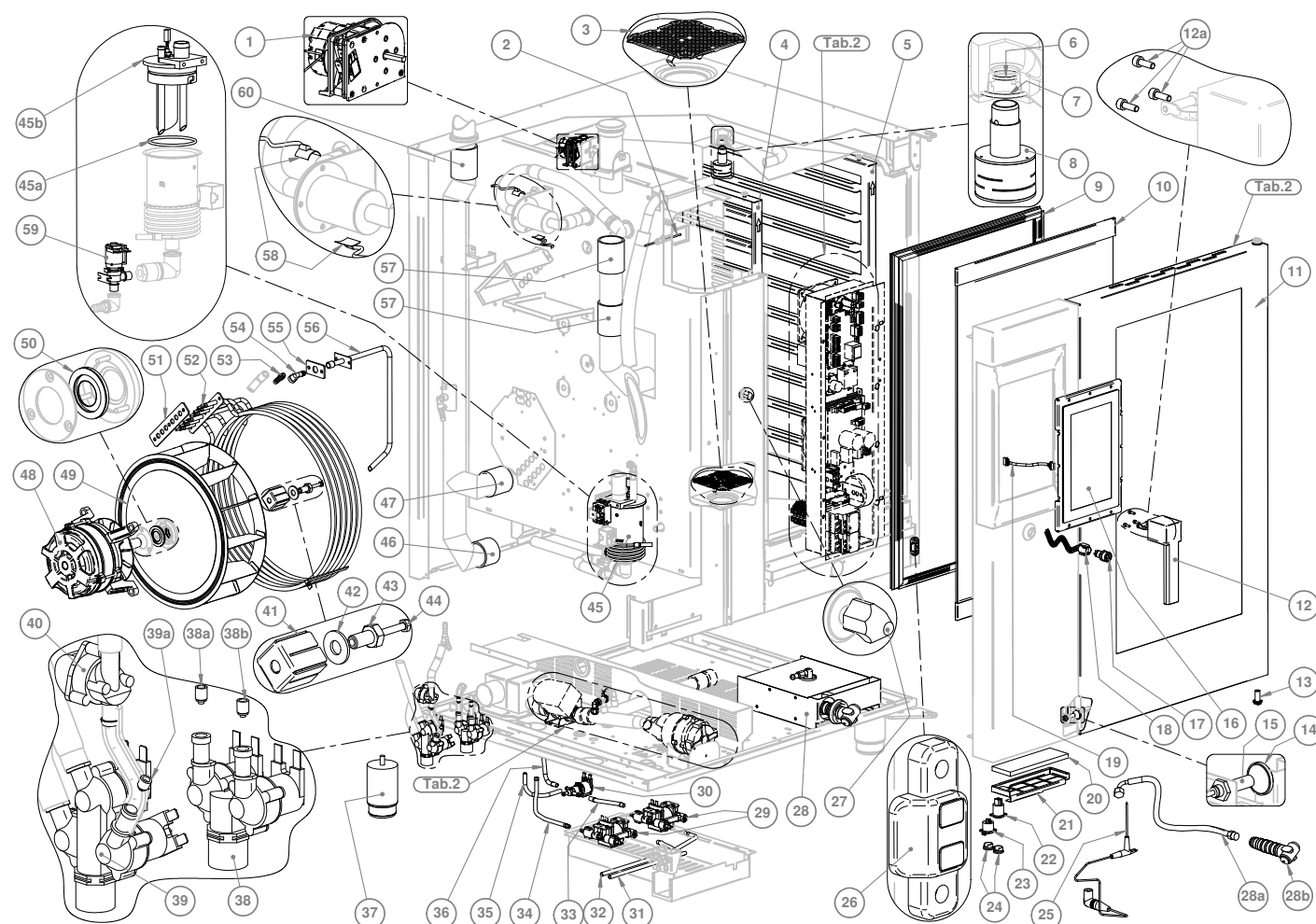
Exploded view 1/2
